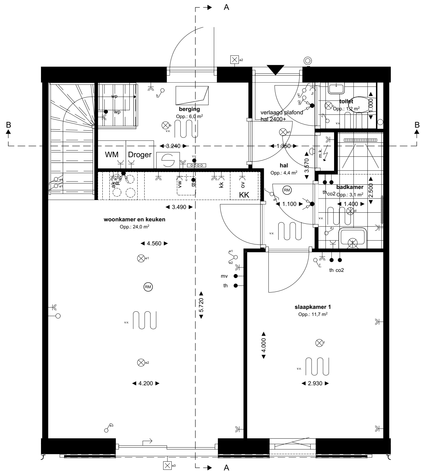
00 Begane grond - 1:50
